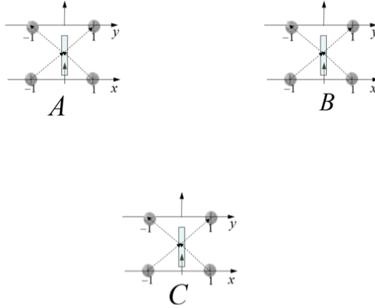
Figure 2: The observers at sites A , B , and C are asked simultaneously to measure \tilde{x} or \tilde{y} of their particles. This is just either testing the presence of the particle at the locations x = \pm 1 , or passing it through the beam splitter, and then testing the presence of the particle at the locations y = \pm 1 . Quantum theory predicts the correlations between the outcomes of these measurements given by equations (5) and (7). Equation (8) shows that these correlations are inconsistent with the assumption that the outcomes of the measurements are predetermined.
