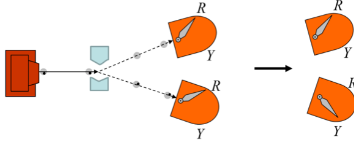
Figure 5: When the standard quantum theory predicts an equal probability for the results of the Stern-Gerlach experiment, the Bohmian position in the lower half of the wave packet of the particle ensures that it will be detected by the lower detector. Depending on the type of the Stern-Gerlach magnet, this will correspond to the results: spin “down” or spin “up”. ( R refers to READY position and Y to YES position of the pointer which signifies detection of the particle.)
