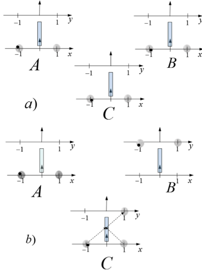
Figure 6: All Bohmian positions in the GHZ setup are placed in the wave packets \tilde{x} = -1 . This ensures \tilde{x}_A = \tilde{x}_B = \tilde{x}_C = -1 and \tilde{y}_A = \tilde{y}_B = \tilde{y}_C = -1 if only one of the measurements is performed and the beam splitters are chosen with \tilde{y} = 1 on the right. b) After the measurement of \tilde{y}_B (passing of the wave packets through the beam splitter is enough) the conditional wave function of the particle in C collapses to |\tilde{y}_C\rangle = 1 . This ensures fulfillment of \tilde{x}_A \tilde{y}_B \tilde{y}_C = 1 .
