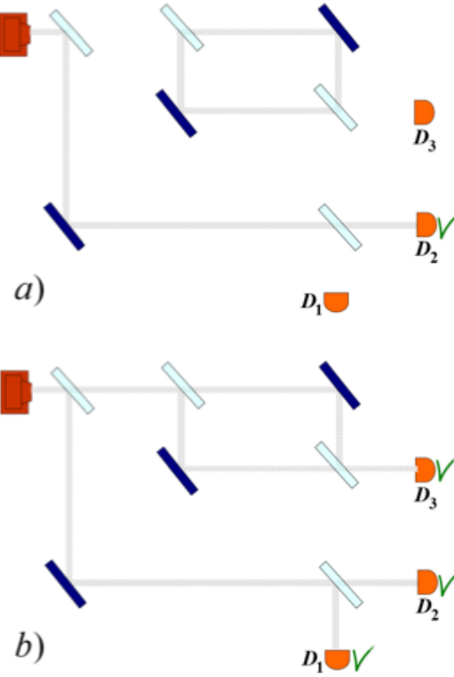
Figure 9: (a). The weak trace left by the photon entering the interferometer in the world in which it was detected in detector D_2 . (b). The weak trace left by the photon in the physical Universe.
