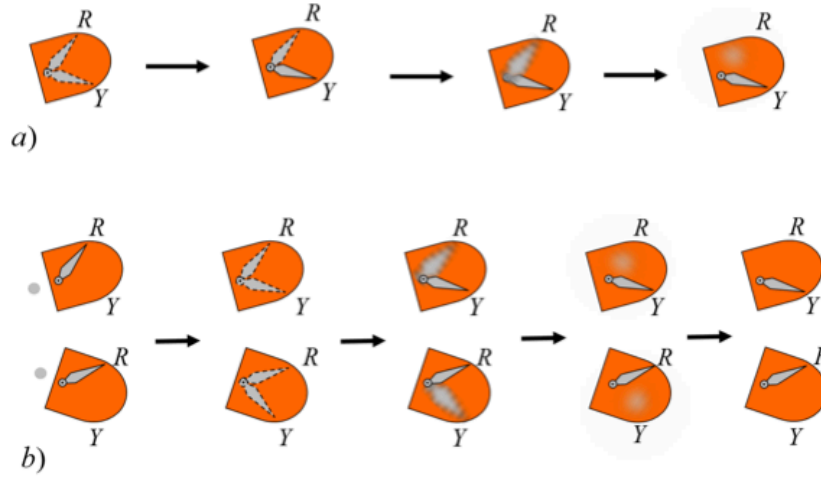
Figure 4: The dynamics of the GRW collapse of the wave function of the pointer in superposition. The first GRW hit collapses the amplitude of the tail pointer state to a very small number. The following hits quickly destroy the tail state of the pointer such that the pointer disintegrates. b). In the Stern-Gerlach experiment, Fig. 3a, the GRW hits lead to a single stable structure of the pointer's states. ( R refers to READY position and Y to YES position of the pointer which signifies detection of the particle.)
