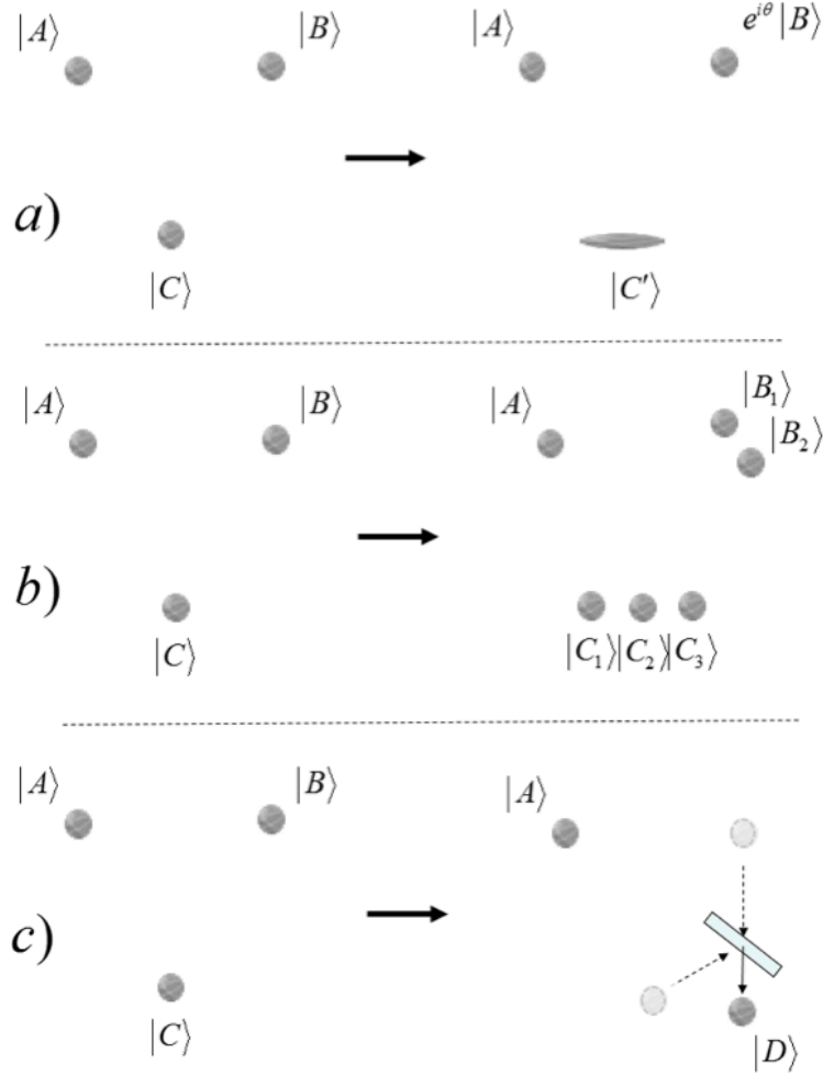
Figure 8: Probability of finding particle in A equal one third due to symmetry. Modifications of states in B and C cannot change the probability in A since there is no action at a distance in quantum theory. a) The wave packet in B gets local phase and the one in C is distorted in space. b) The wave packet in B splits into two identical wave packets and the one in C splits into three. c) Using a beam splitter the wave packets in B and C interfere into one wave packet |D\rangle .
