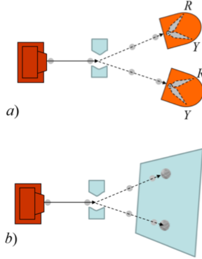
Figure 3: The Stern-Gerlach experiment with pointer displays. R refers to READY position and Y to YES position of the pointer which signifies detection of the atom. The superposition of the wave packets of the atom creates an entangled superposition of the two pointers which collapses almost to a product state due to the first GRW hit. b). The Stern-Gerlach experiment with a screen display. The superposition of the wave packets of the atom creates an entangled superposition of the internal states of a macroscopic number of atoms on the screen. This superposition does not collapse due to the GRW hits, so the definite result of the measurement will take place at a much later stage.
