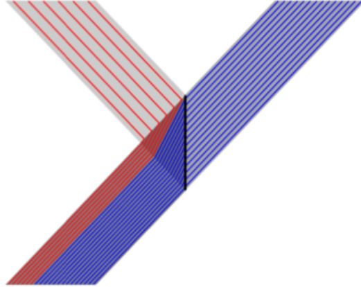
Figure 7: A wave packet passing through a beam splitter, in the Many Bohmian Worlds picture. In this example, there is a chance of 70% to cross the beam splitter. The gray areas represent the incident, transmitted and reflected wave functions. Blue trajectories represent particles which get through the beam splitter, while red trajectories represent reflected particles.
