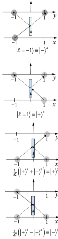
Figure 1: The first two figures show the eigenstates of the variable \tilde{x} which are the wave packets localized at points \pm 1 on the x axis. The two figures in the bottom show the eigestates of the variable \tilde{y} which are superpositions of eigestates of \tilde{x} . They become localized wave packets on a parallel axis (which is named y ) after passing through a vertical beam splitter. The eigenstates of \tilde{x} passing through the beam splitter become superpositions of the wave packets localized at \pm 1 on the y axis.
